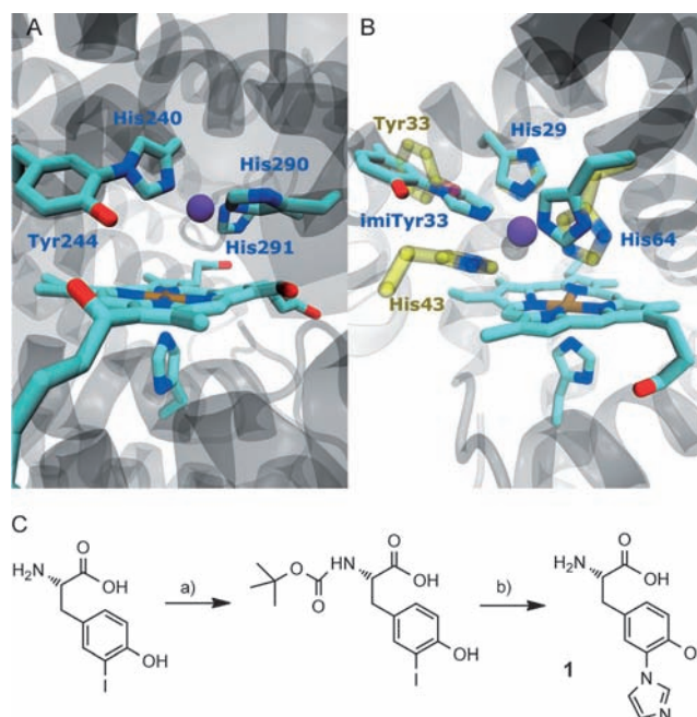
Figure 1. A) Cu B site of cytochrome c oxidase (bovine numbering). B) Structure model overlay of imiTyrCu B Mb (cyan) and F33YCu B Mb (yellow). C) Synthesis of imiTyr ( 1 ). a) Di-tert-butyl dicarbonate, THF, 1 N NaOH, RT, 4 h. b) Imidazole, Cs 2 CO 3 , CuI, DMF, reflux, 16 h. Color code in (A) and (B): Cu pink, N blue, O red, Fe brown.
